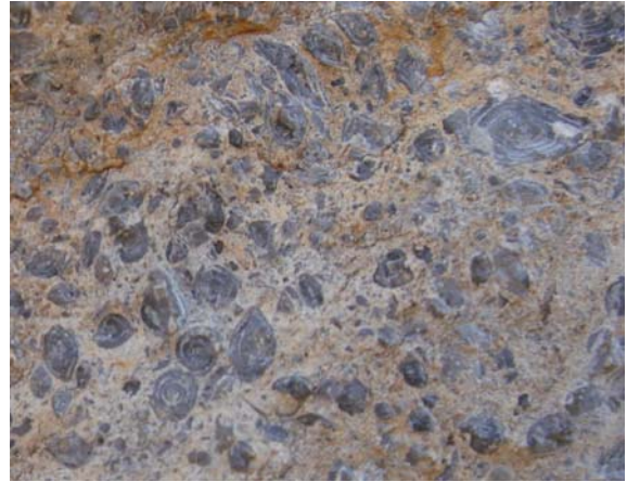
Fusulina in the limestone (The wall of Taxila ruin)
