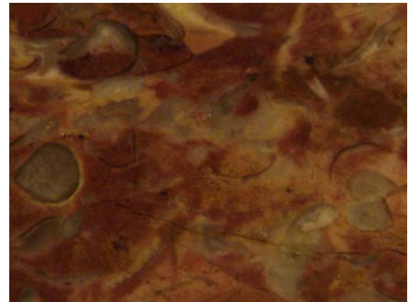
Fusulina in the marble (hotel floor)
